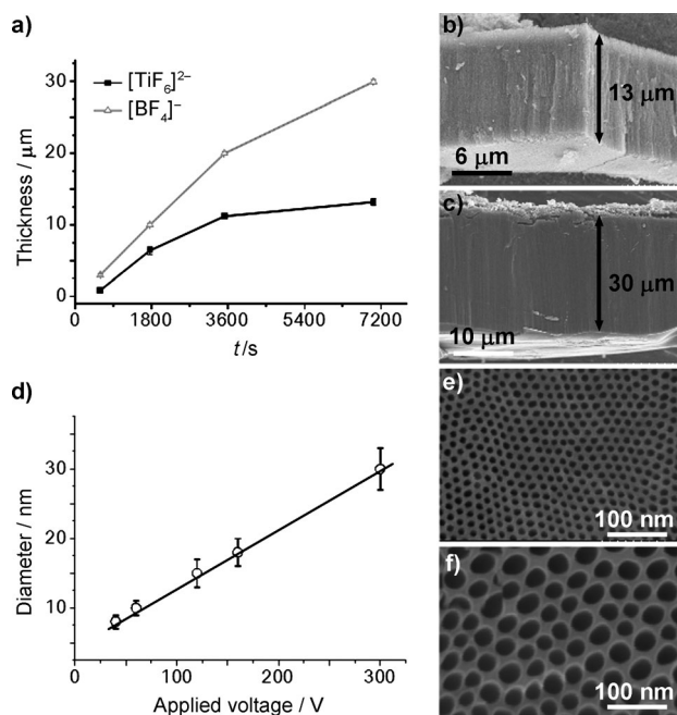
Figure 2. a) Time–thickness curves of nanoporous V_2O_5 layers anodically grown in [TiF_6]^{2-} and [BF_4]^- -containing electrolytes (squares: 300 ppm Ti electrolyte dissolved in EG, triangles: 14 mM NaBF_4 electrolyte with 3 M H_2O in EG). b,c) SEM images of the porous layers anodically formed in [TiF_6]^{2-} and [BF_4]^- -containing electrolytes at 120 V for 2 h, respectively. d) Applied voltage–diameter curve of the porous layer anodically grown in Ti (300 ppm) electrolyte. e,f) SEM images of the porous layers formed at 40 and 300 V, respectively.
